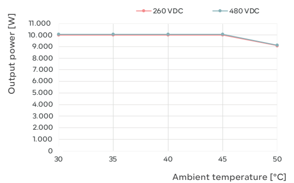
Fronius Primo GEN24 10.0 208-240 [Plus] Temperature derating (240VAC)
