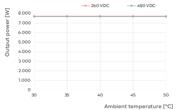
Fronius Primo GEN24 7.7 208-240 [Plus] Temperature derating (240VAC)
